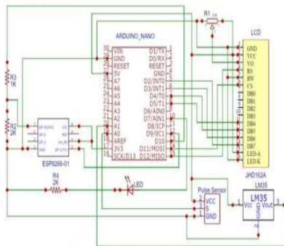
Figure 4. Circuit Schematic Diagram.
